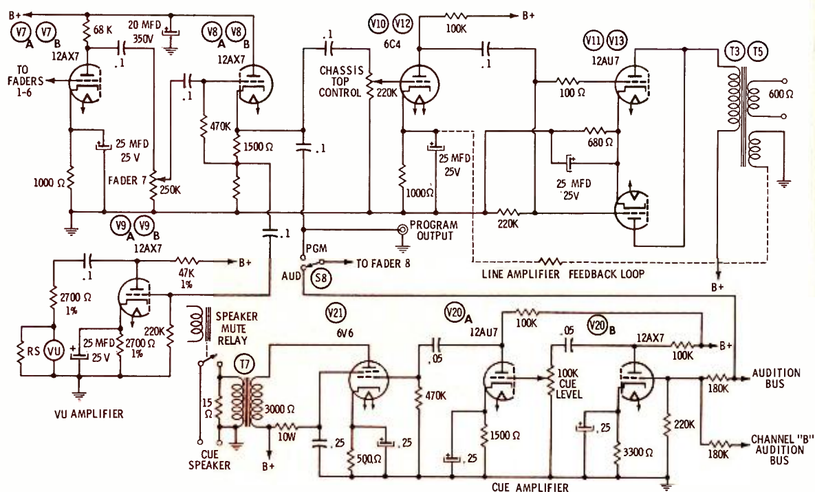
Fig. 5. Schematic diagram shows circuit arrangement and parts values of cue amplifier and one of the two-main channel amplifiers.
