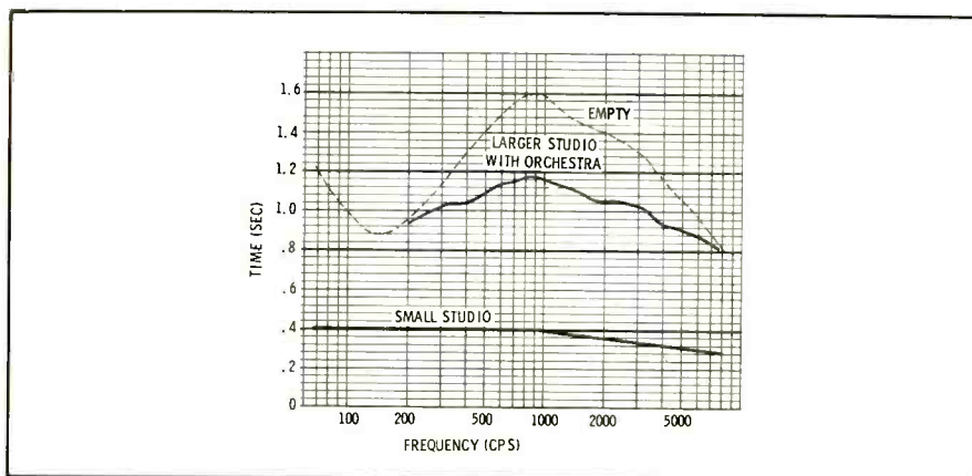
Fig. 3. Reverberation time depends on size and occupancy as well as frequency.
