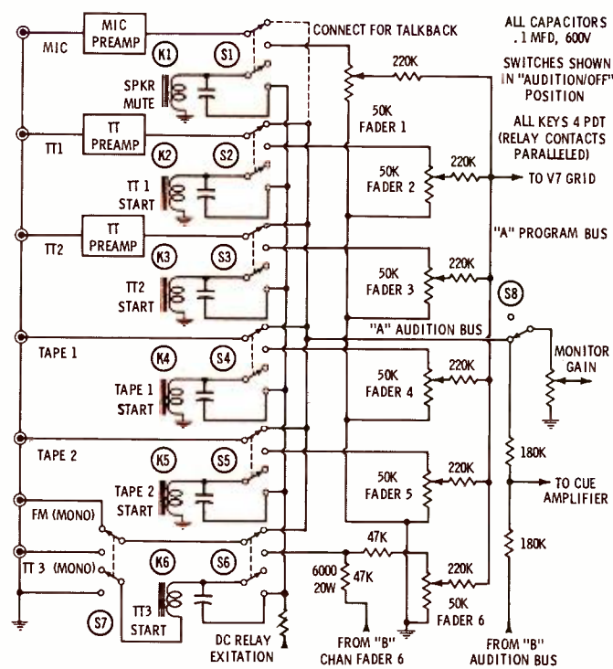
Fig. 4. Switching section controls both audio, stop-start relays (one channel shown).
