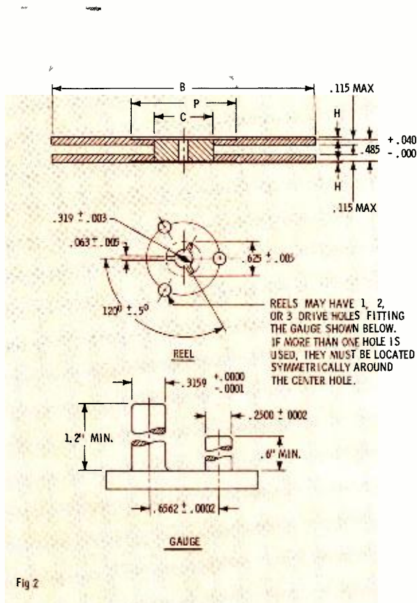
Fig. 2. Dimensions specified in Standard for NAB Type B reels.
