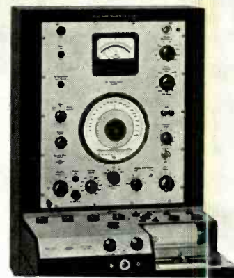
Fig. 5. Automatic frequency-response recorder can measure reverberation time.
