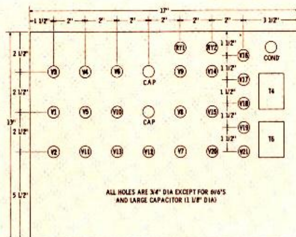
Fig. 9. Typical tube and transformer layout for the portable stereo consolette.
