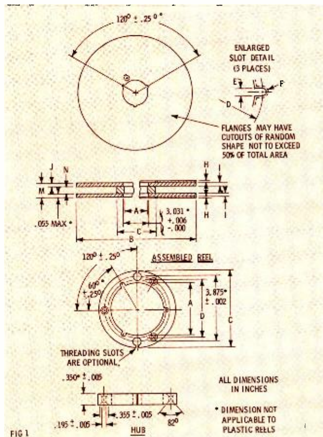
Fig. 1. Dimensions specified in Standard for NAB Type A reels.
