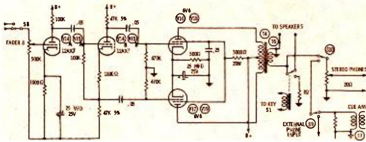
Fig. 6. One of the two identical monitor amplifiers for use in the stereo consolette.
