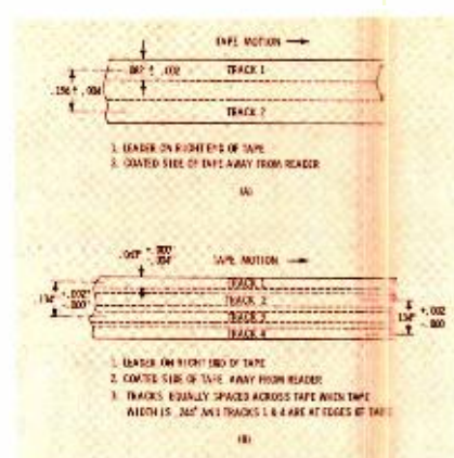
Fig. 3. Standard tape-track designations.
