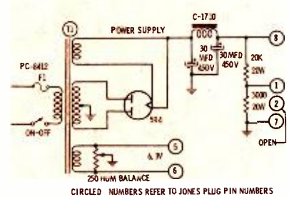
Fig. 7. Circuit of outboard power supply.
