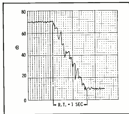
Fig. 6. Typical decay curve for a pure tone source shows reverberation time.
