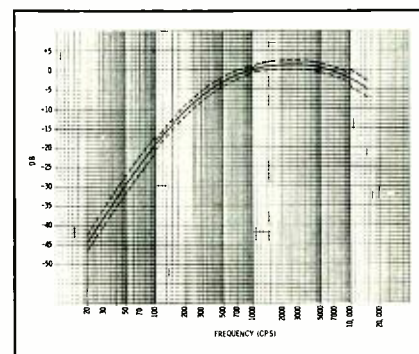
Fig. 6. Weighted noise measurement curve.
