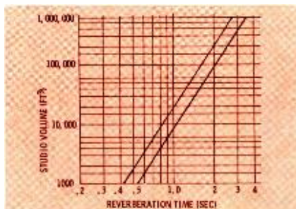
Fig. 2. Graph relating studio volume and recommended reverberation-time range.
