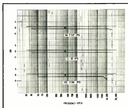
Fig. 5. Recording frequency response.
