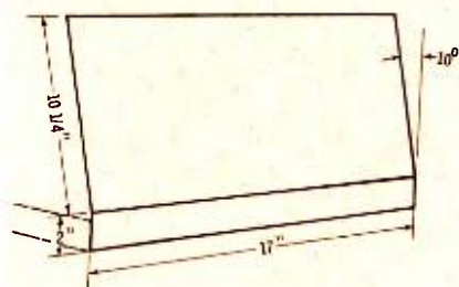
Fig. 8. Dimensions for bending the panel.
