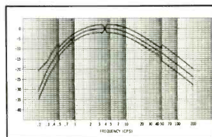
Fig. 7. Flutter measurement weighting.
