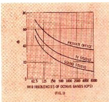
Fig. 1. Noise-rating curves (Kosten and Van Os) for three different environments.
