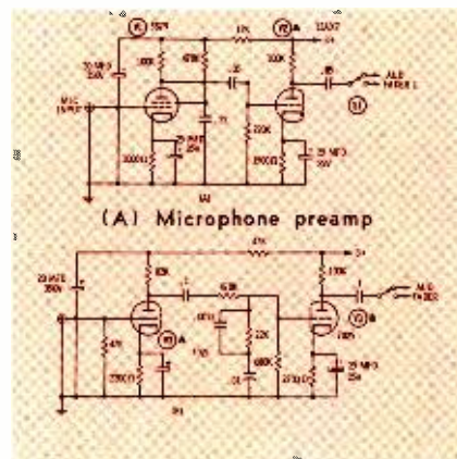
Fig. 3. Preamplifier schematic diagrams.
