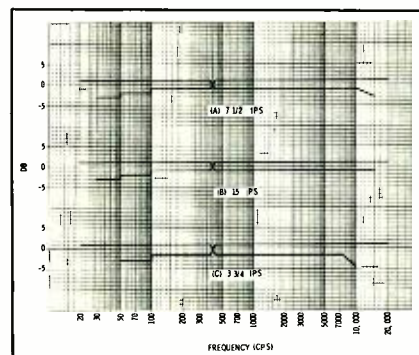
Fig. 4. Reproducing frequency response.
